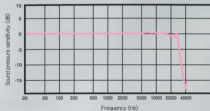
● Frequency characteristics of microphone (TYPE 7052NR)
