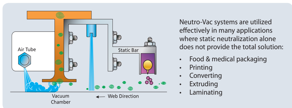
Neutro-Vac Brush Contact Head with Static Bars & Air Tube (available without a brush as a non-contact version)
